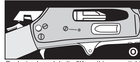
Replacing breech bolt (*Keep this screw tight)
